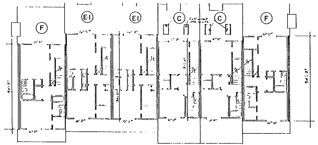
SECOND FLOOR PLAN BUILDING (M)
