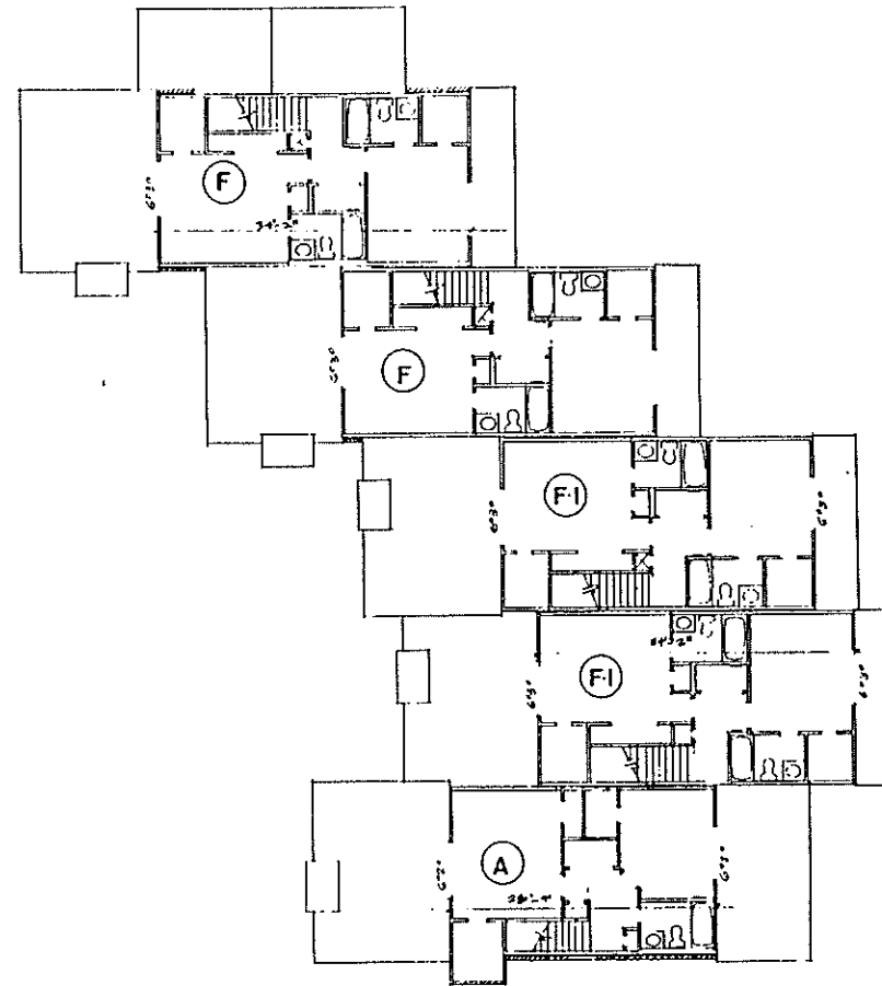
SECOND FLOOR PLAN BUILDING (L)
