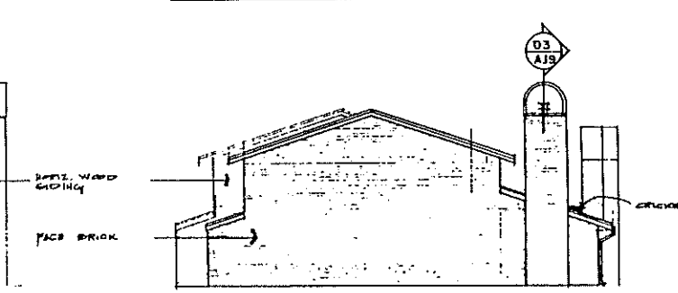
END ELEVATION BLDG. (M)
