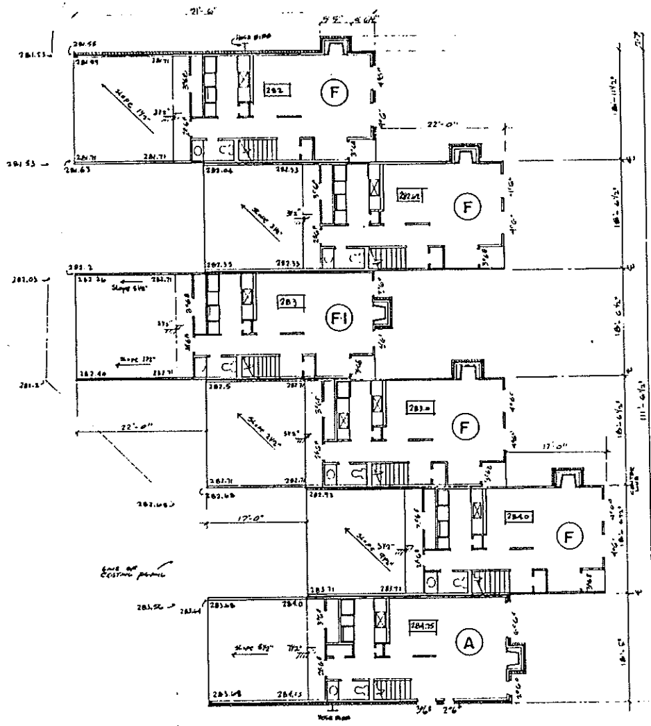
FIRST FLOOR PLAN BUILDING (K)
