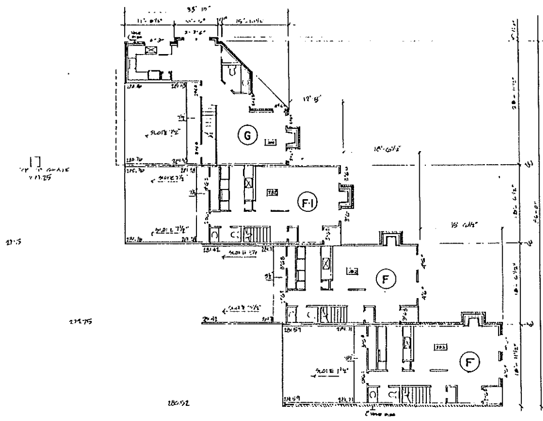
FIRST FLOOR PLAN BUILDING (N)
