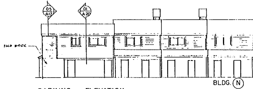
PARKING ELEVATION
