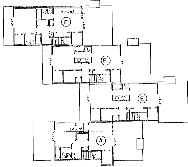
SECOND FLOOR PLAN BUILDING (O)
