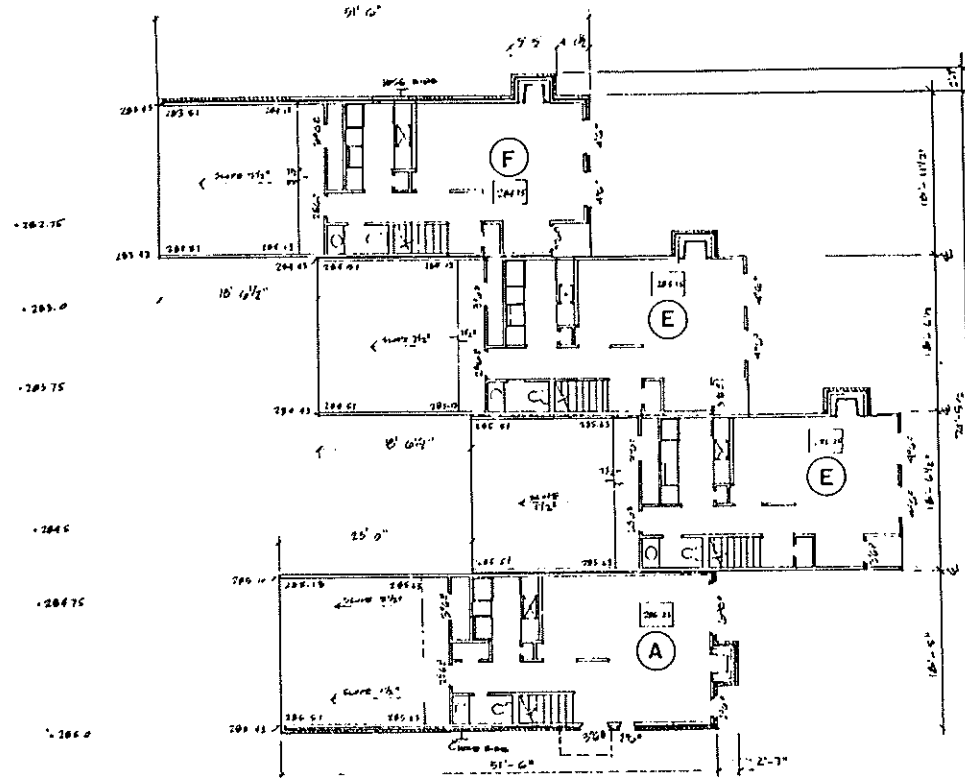
FIRST FLOOR PLAN BUILDING (O)
