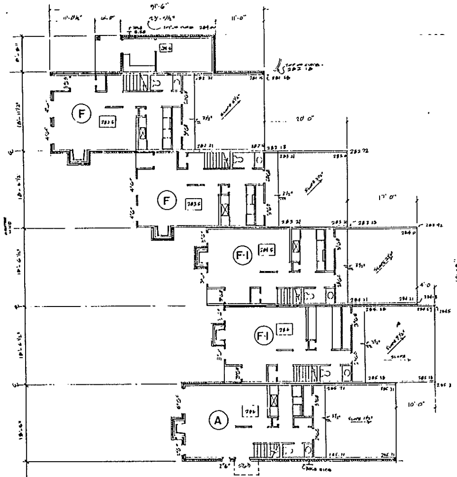
FIRST FLOOR PLAN BUILDING (L)
