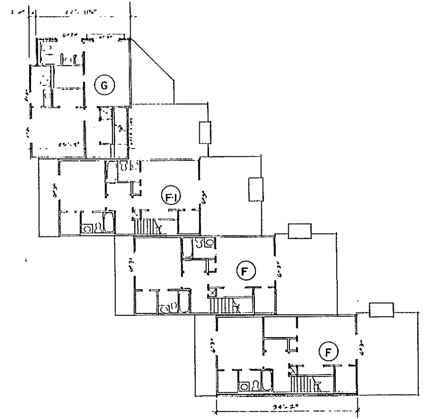
SECOND FLOOR PLAN BUILDING (N)
